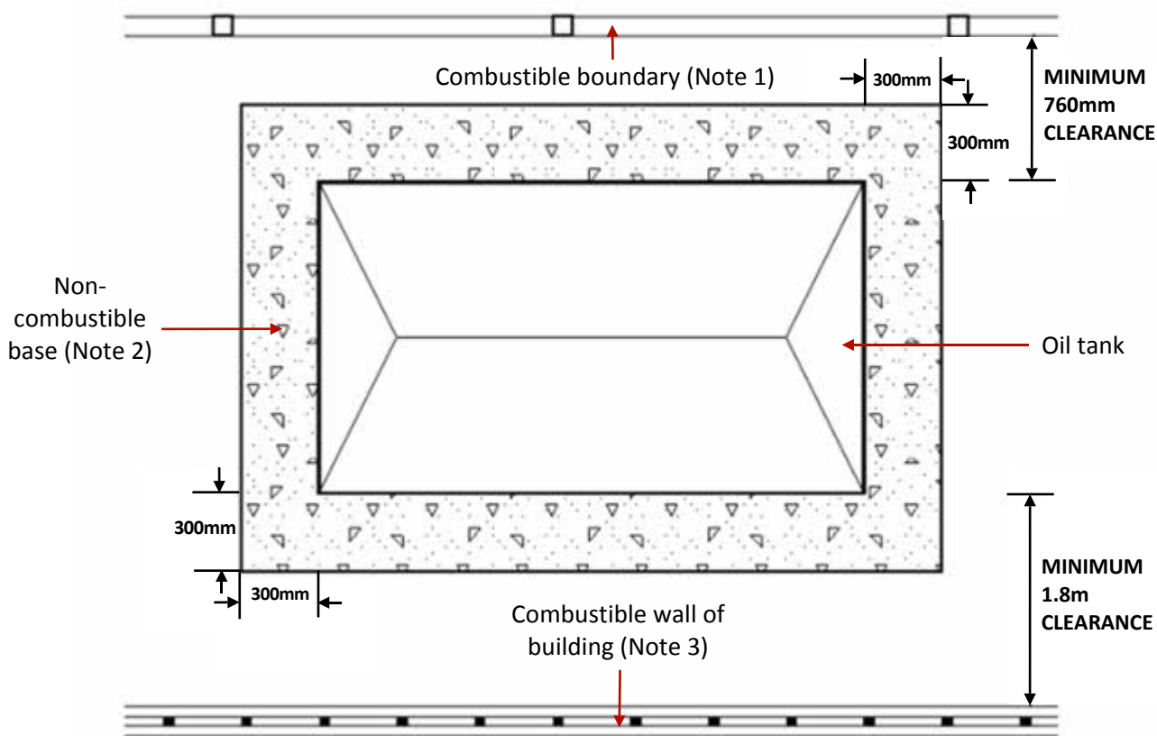
Figure 4: Oil Tank Installation Near Combustible Buildings & Boundaries
